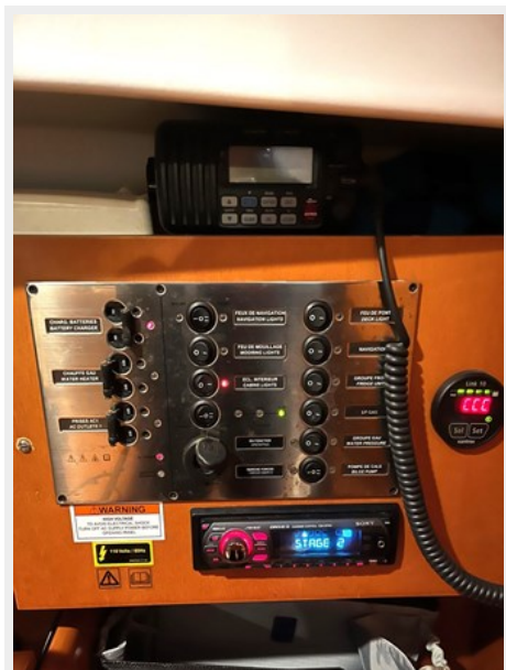
Nav panel IMG_2094
