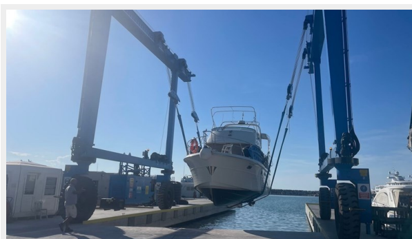
Travel lift
