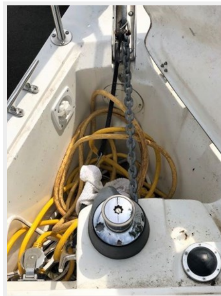
thumbnail_Anchor locker details IMG_5125
