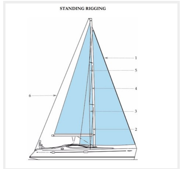
Sail plan
