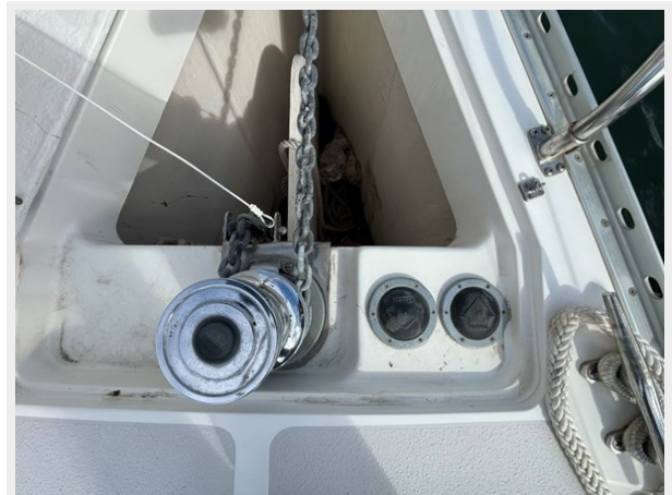
Electric Windlass
