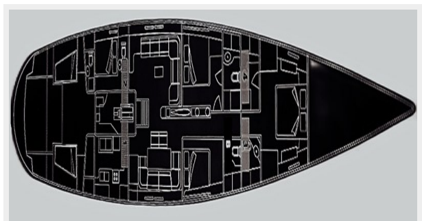
Layout Fancy_WindYachts
