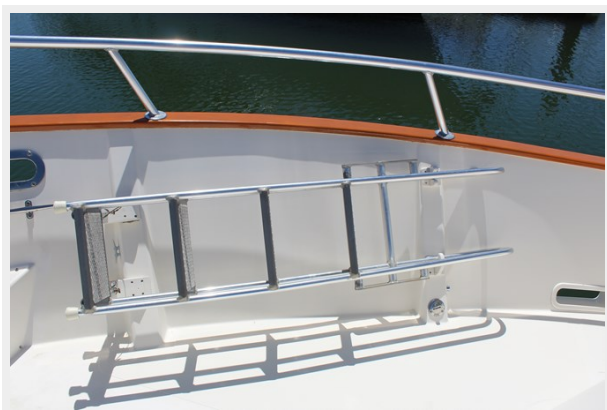
Bow storage for custom side boarding ladder
