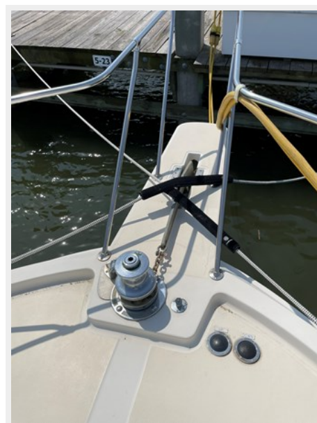
Anchor/Windlass
