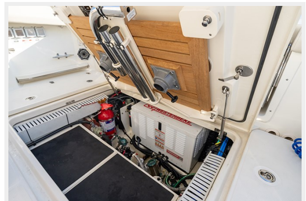
Engine compartment
