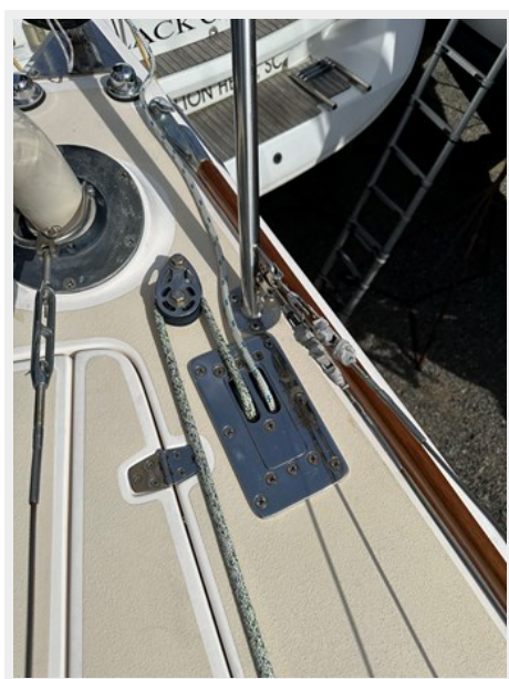
Foredeck Detail
