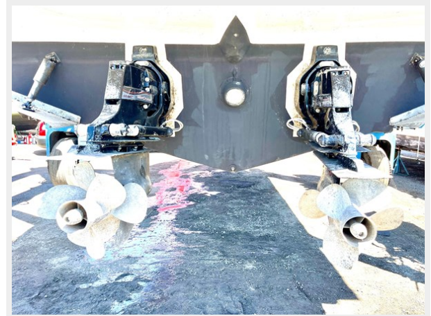
Out Drives
