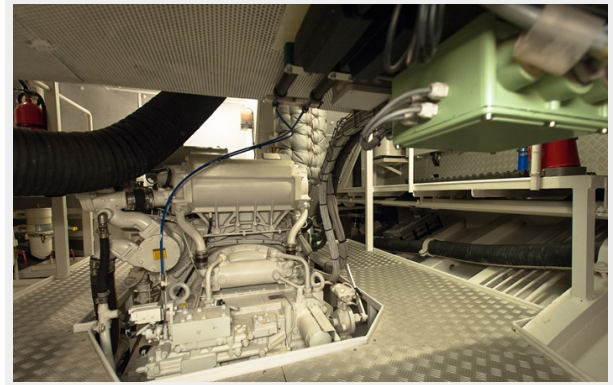
ATLANTIC Engineeroom
