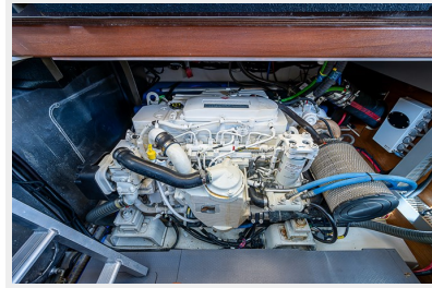
47_beneteau_swift_trawler_horizon_iv_engine_room_3
