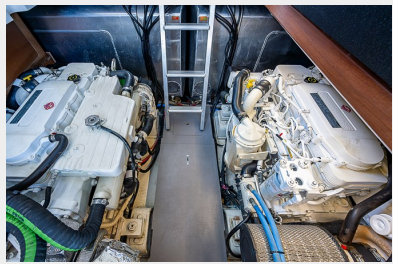
47_beneteau_swift_trawler_horizon_iv_engine_room_4
