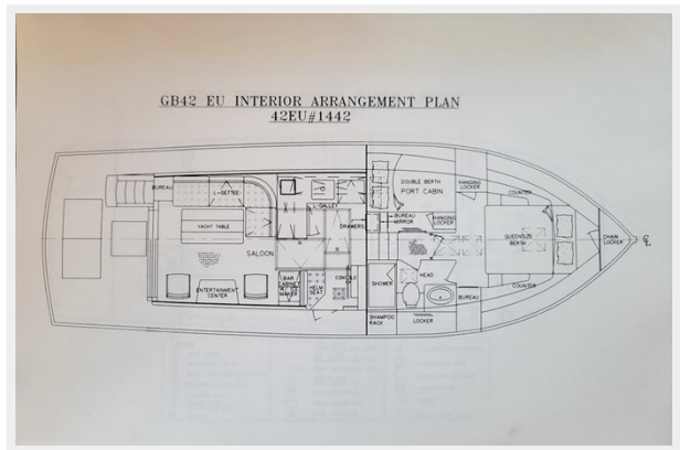
GA Layout
