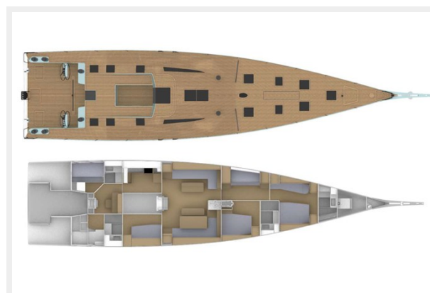
General Arrangement
