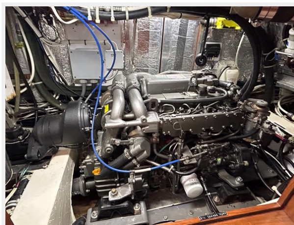
Engine, Side
