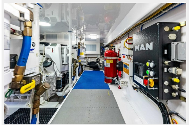
2021 Viking 54 Convertible
