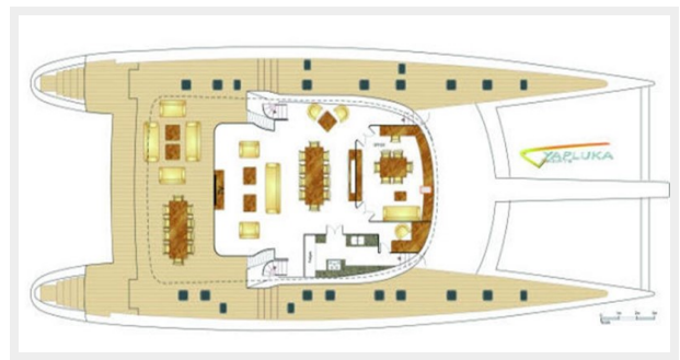
Main Deck
