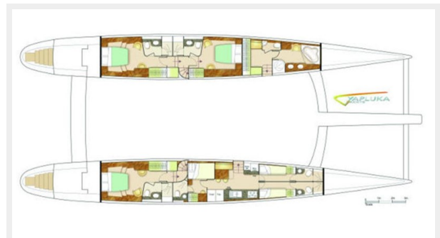
Hull Layout
