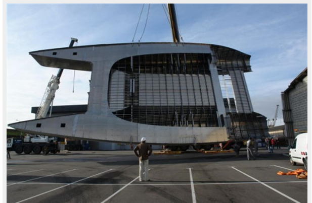
Turning of Hulls
