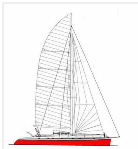
Sailplan
