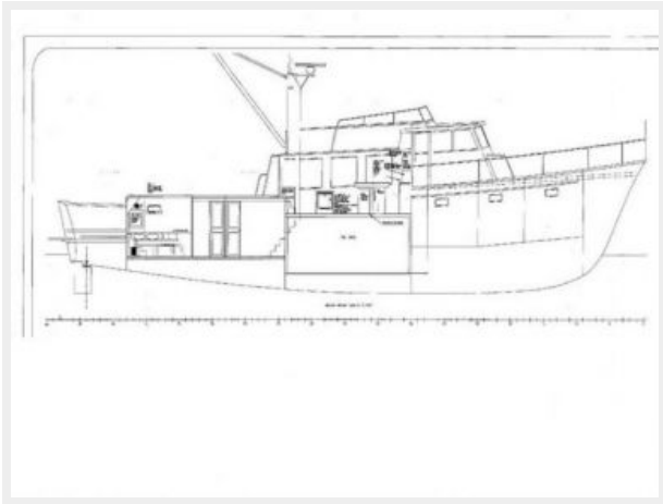
Layout
