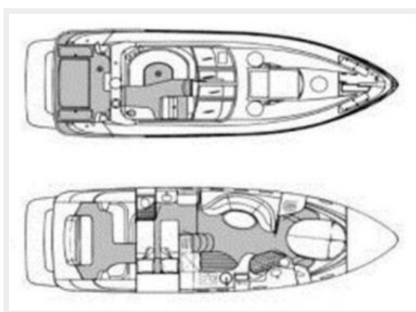
Regal 4260 Layout
