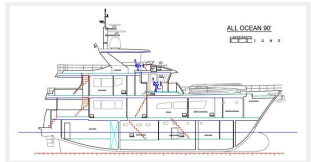
Cutway View
