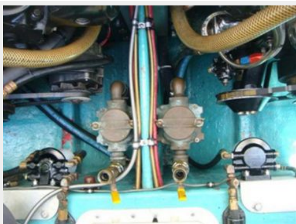
Engine Compartment
