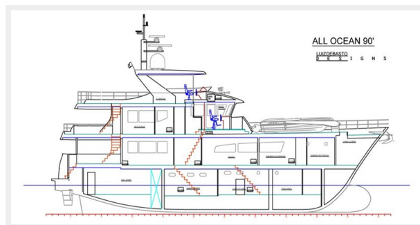
Cutway View
